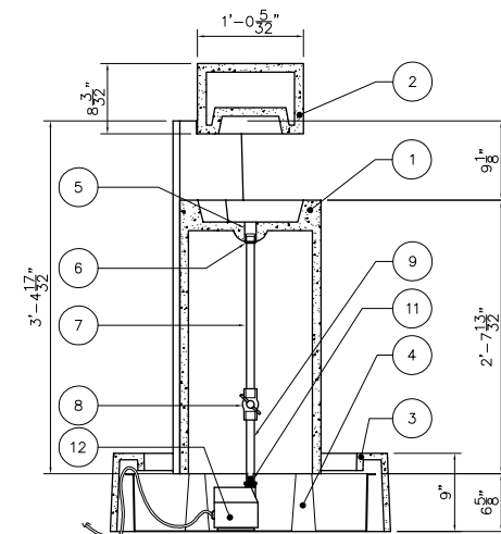
3 SECTION
