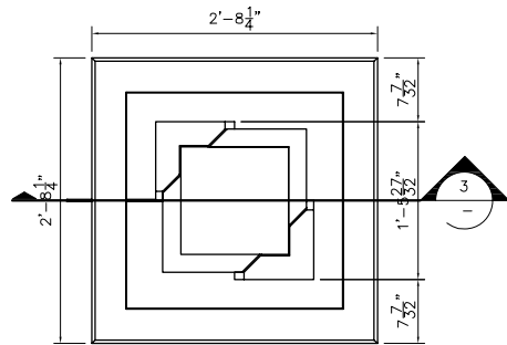
1 PLAN VIEW
